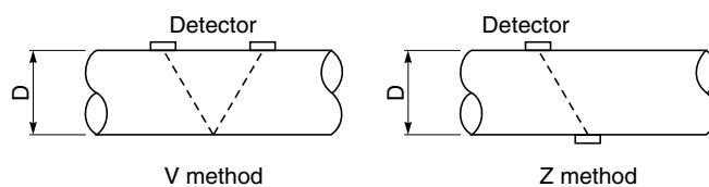
Fig. 2-2 Mounting method
