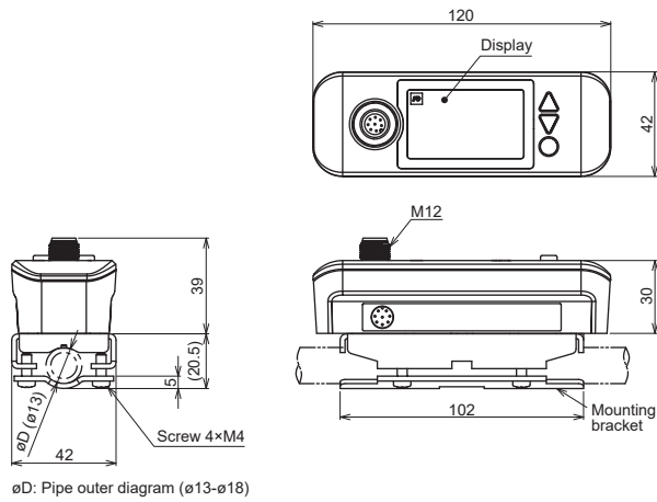
Type: FSZ08
