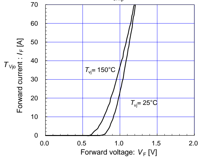
Forward current vs. Forward voltage (typ.) chip
