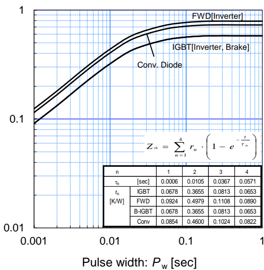
Transient thermal Impedance (max.)
