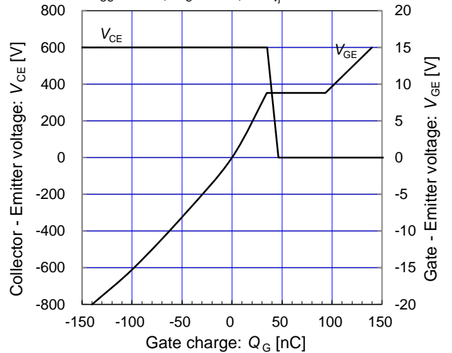
Dynamic Gate charge (typ.) V_{CC} = 600\text{V}, I_C = 35\text{A}, T_{vj} = 25^{\circ}\text{C}
