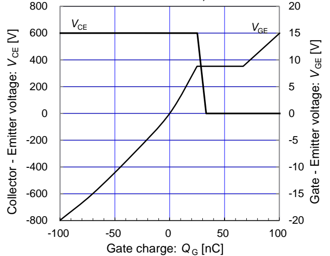
Dynamic Gate charge (typ.) V_{CC} = 600\text{V}, I_c = 25\text{A}, T_{vj} = 25^{\circ}\text{C}
