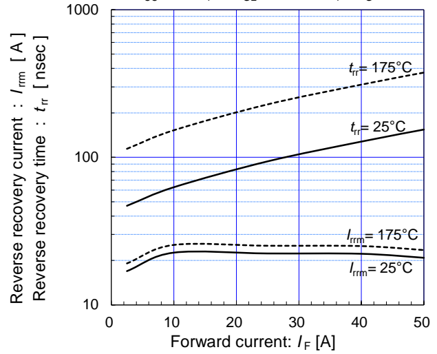
Reverse recovery characteristics (typ.) V_{CC}=600V, V_{GE}=+15/-15V, R_G=20\Omega
