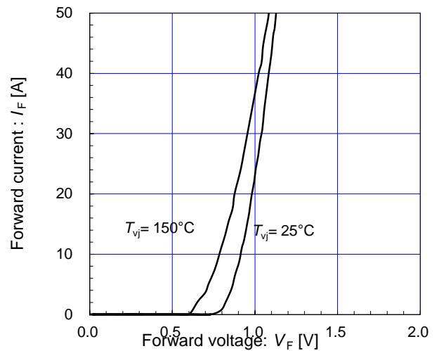
Forward current vs. Forward voltage (typ.) chip
