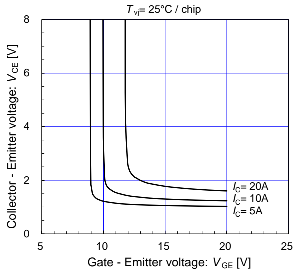
Collector-Emittor voltage vs. Gate-Emittor voltage (typ.)
