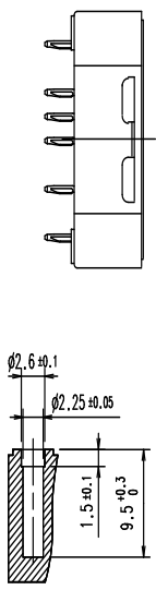
断面A-A (1.5:1) SECTION A-A Weight: 25 g (typ.)
