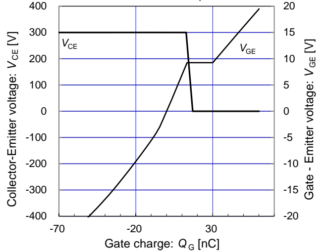
Dynamic Gate charge (typ.) V_{CC} = 300\text{V}, I_c = 10\text{A}, T_{vj} = 25^{\circ}\text{C}
