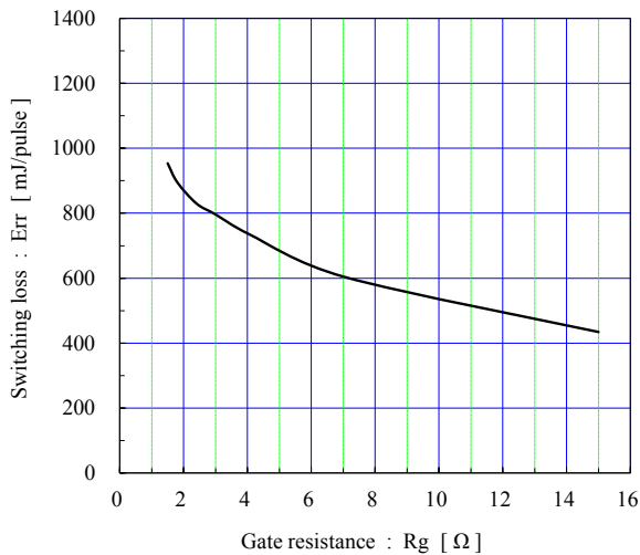
Switching loss vs. Gate resistance (typ.) V_{CC}=1800V, I_F=800A, V_{GE}=\pm 15V, T_j=125^\circ C
