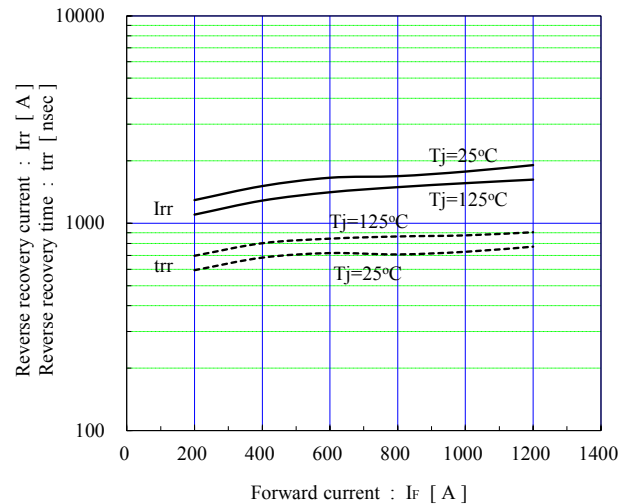
Reverse recovery characteristics (typ.) V_{CC}=1800V, V_{GE}=\pm 15V, R_g=2.4\Omega
