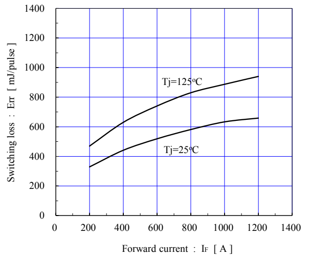
Switching loss vs. Collector current (typ.) V_{CC}=1800V, V_{GE}=\pm 15V, R_g=2.4\Omega
