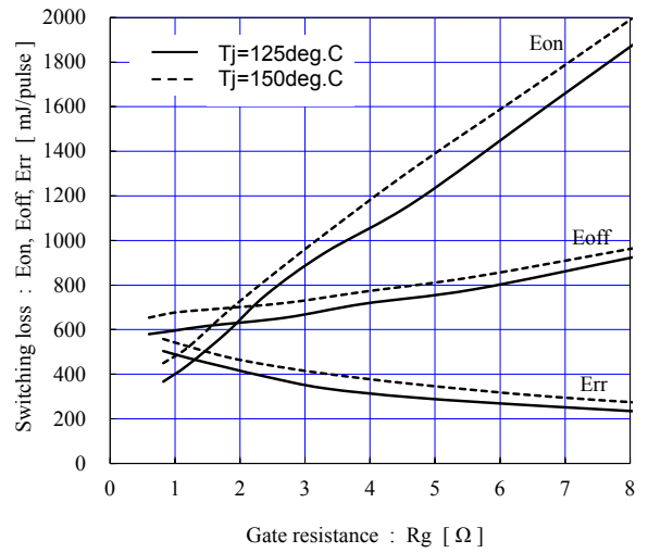
Switching loss vs. Gate resistance (typ.) V_{cc}=900V, I_c=1600A, V_{GE}=\pm 15V
