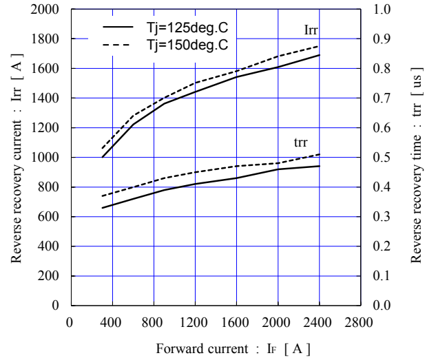
Reverse recovery characteristics (typ.) V CC =900V, V GE =±15V, R gon =1.4Ω
