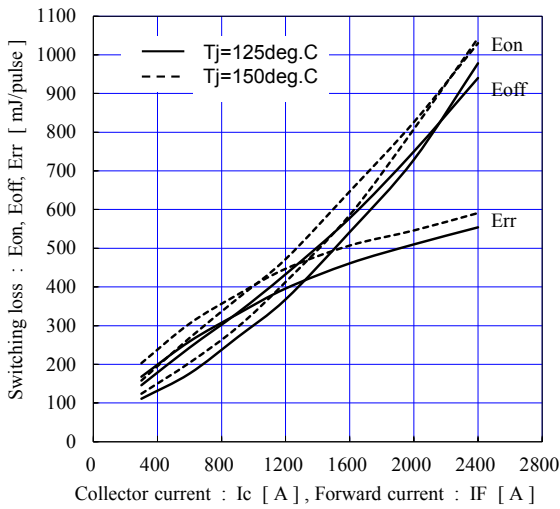
Switching loss vs. Collector current (typ.) V_{cc}=900V, V_{GE}=\pm 15V, R_{gon}=1.4\Omega, R_{goff}=0.6\Omega
