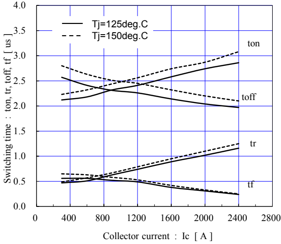
Switching time vs. Collector current (typ.) V_{cc}=900V, V_{GE}=\pm 15V, R_{gon}=1.4\Omega, R_{goff}=0.6\Omega
