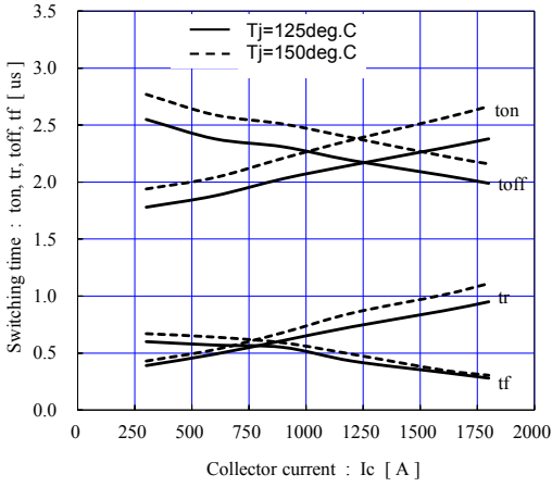
Switching time vs. Collector current (typ.) V_{cc}=900V, V_{GE}=\pm 15V, R_{gon}=1.2\Omega, R_{goff}=0.82\Omega
