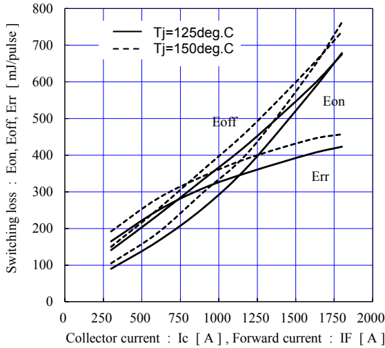
Switching loss vs. Collector current (typ.) V_{cc}=900V, V_{GE}=\pm 15V, R_{gon}=1.2\Omega, R_{goff}=0.82\Omega
