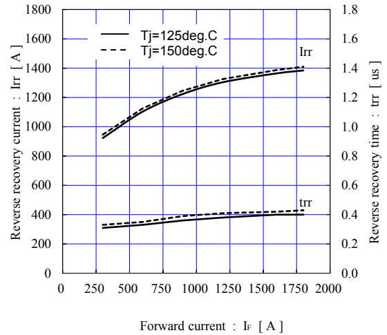
Reverse recovery characteristics (typ.) Vce=900V, VGE=±15V, Rgon=1.2Ω
